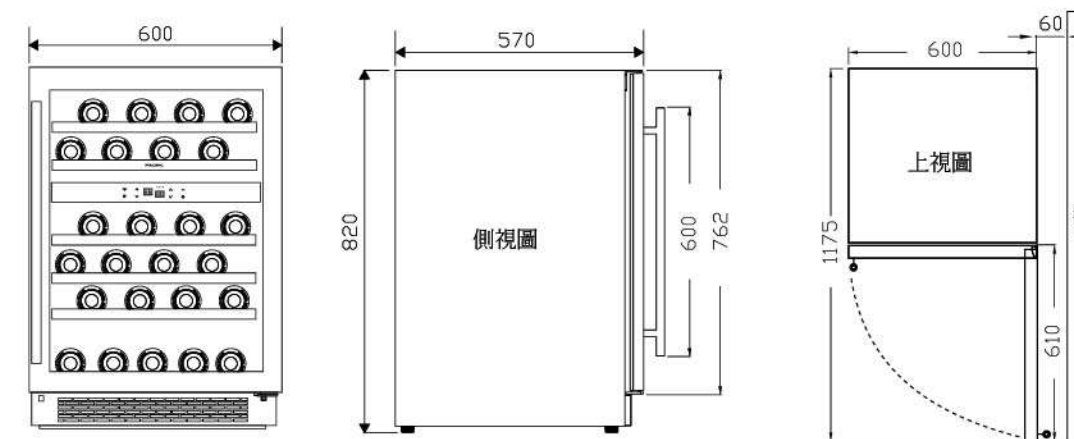
LRW60S 櫥下式單門雙溫紅酒櫃
