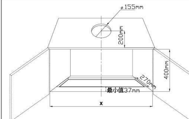
PQ-M60/75/90/120 BST 櫥櫃開孔尺寸
