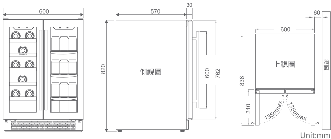
LRW60D 櫥下式雙門雙溫紅酒櫃
